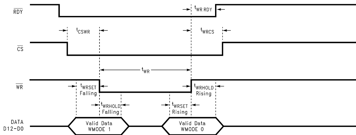
Figure 21. Write Signal Negates \overline{RDY} (Writing the Standby, Auto-Cal or Auto-Zero Command)
